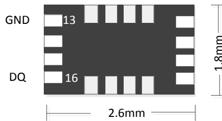
UT_QFN(Bottom View)
