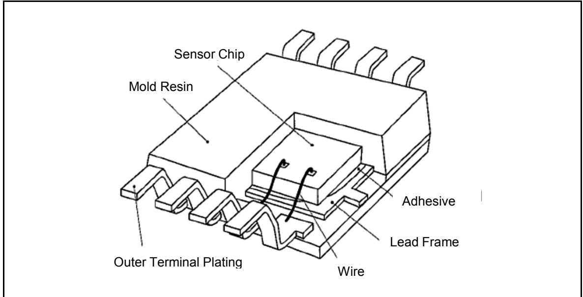
Figure 4-4 Internal Structure
