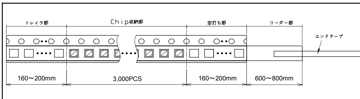
Figure 5-5 Taping Specification
