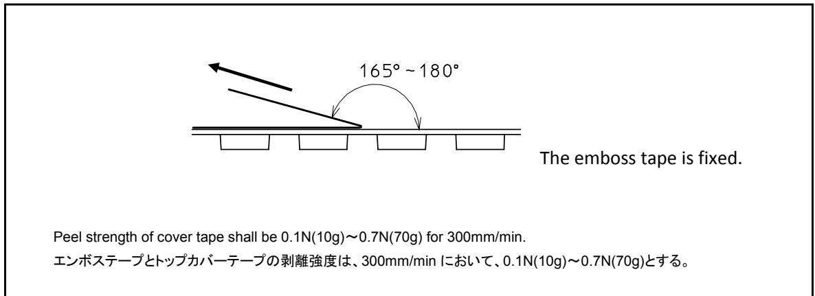
Figure 5-6 Peel Strength
