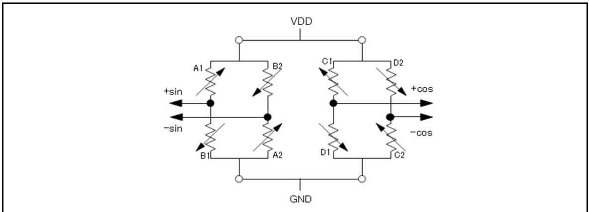
Figure 3-2 Equivalent Circuit
