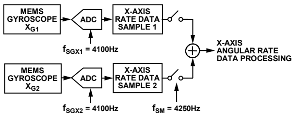
Figure 14. Gyroscope Data Sampling
