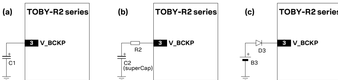
Figure 38: Real time clock supply (V_BCKP) application circuits: (a) using a 100 \mu F capacitor to let the RTC run for ~80 s after VCC removal; (b) using a 70 mF capacitor to let RTC run for ~15 hours after VCC removal; (c) using a non-rechargeable battery
