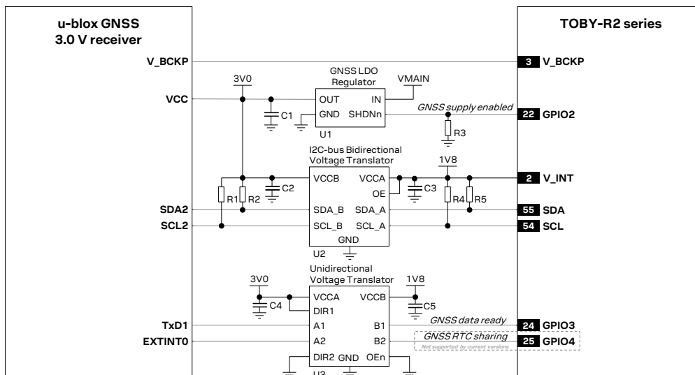
Figure 64: Application circuit for connecting TOBY-R2 series modules to u-blox 3.0 V GNSS receivers
