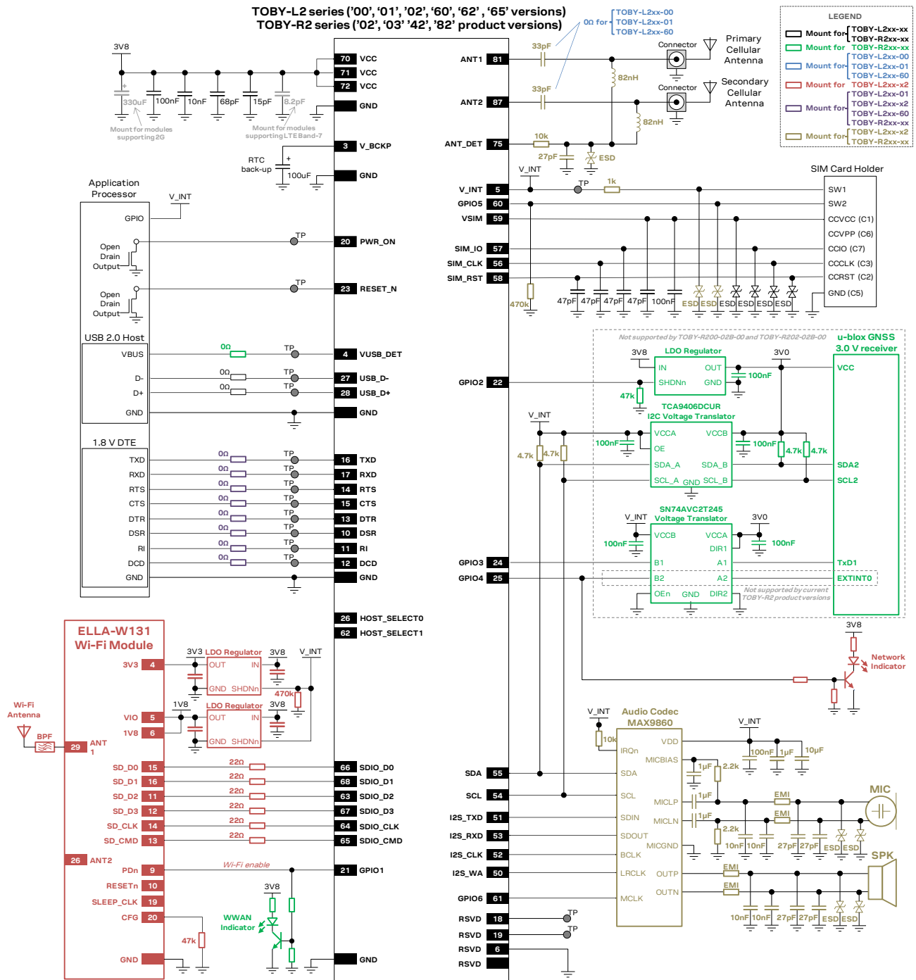
Figure 76: Example of complete schematic diagram to integrate TOBY-L2 modules and TOBY-R2 modules (“00”, “01”, “x2” product versions) on the same application board, using all the available interfaces / functions of the modules
