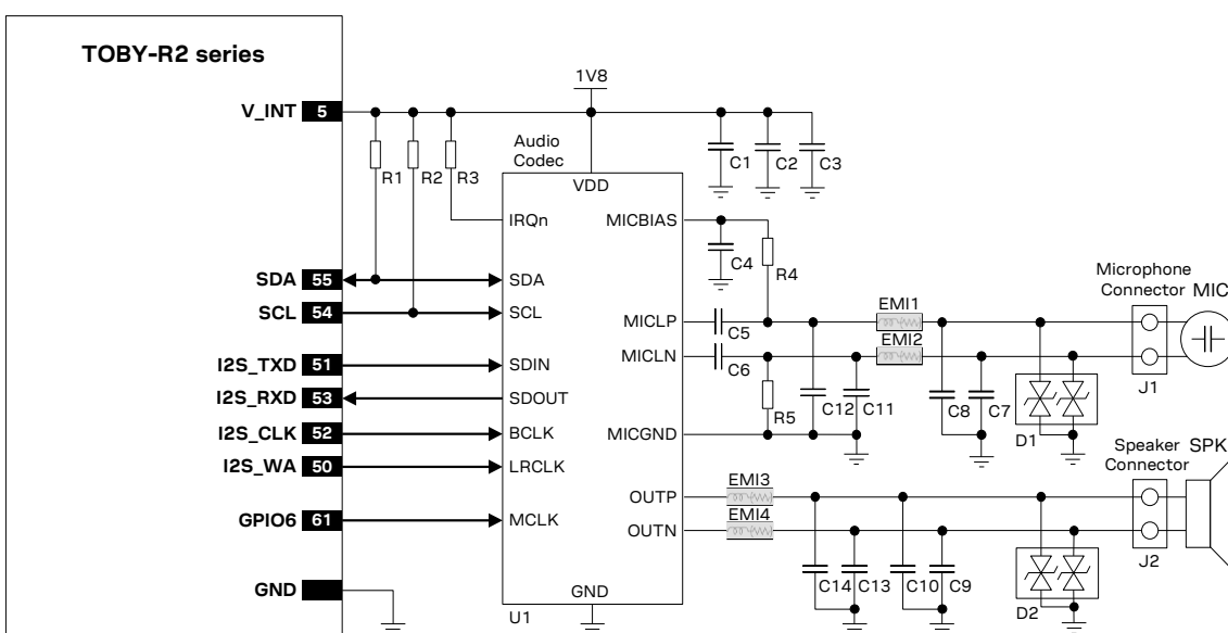
Figure 65: I2S interface application circuit with an external audio codec to provide voice capability
