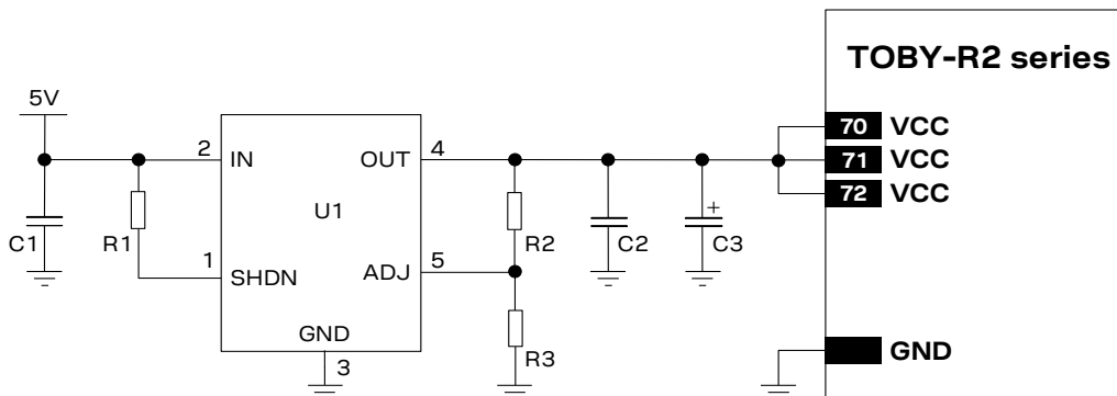
Figure 30: Example of high reliability VCC supply application circuit using an LDO linear regulator
