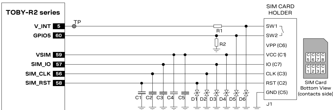
Figure 49: Application circuit for the connection to a single removable SIM card, with SIM detection implemented
