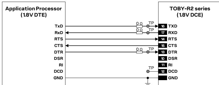
Figure 53: UART interface application circuit with partial V.24 link (6-wire) in the DTE/DCE serial communication (1.8 V DTE)
