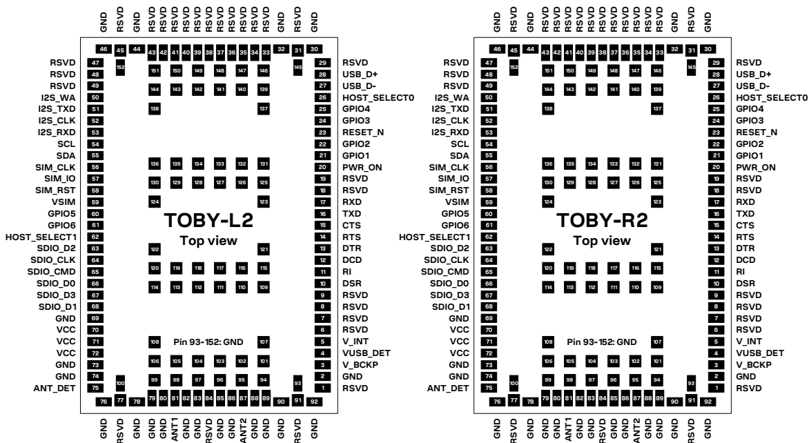
Figure 73: TOBY-L2 and TOBY-R2 series modules pad layout and pin assignment
