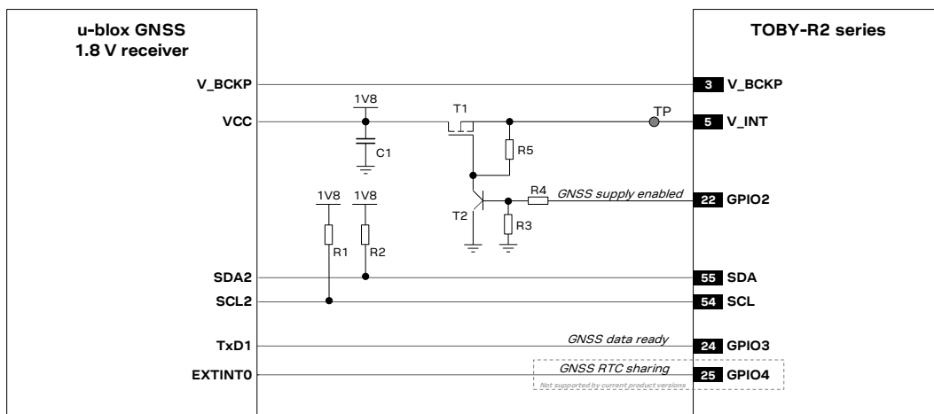
Figure 63: Application circuit for connecting TOBY-R2 series modules to u-blox 1.8 V GNSS receivers using V_INT as supply
