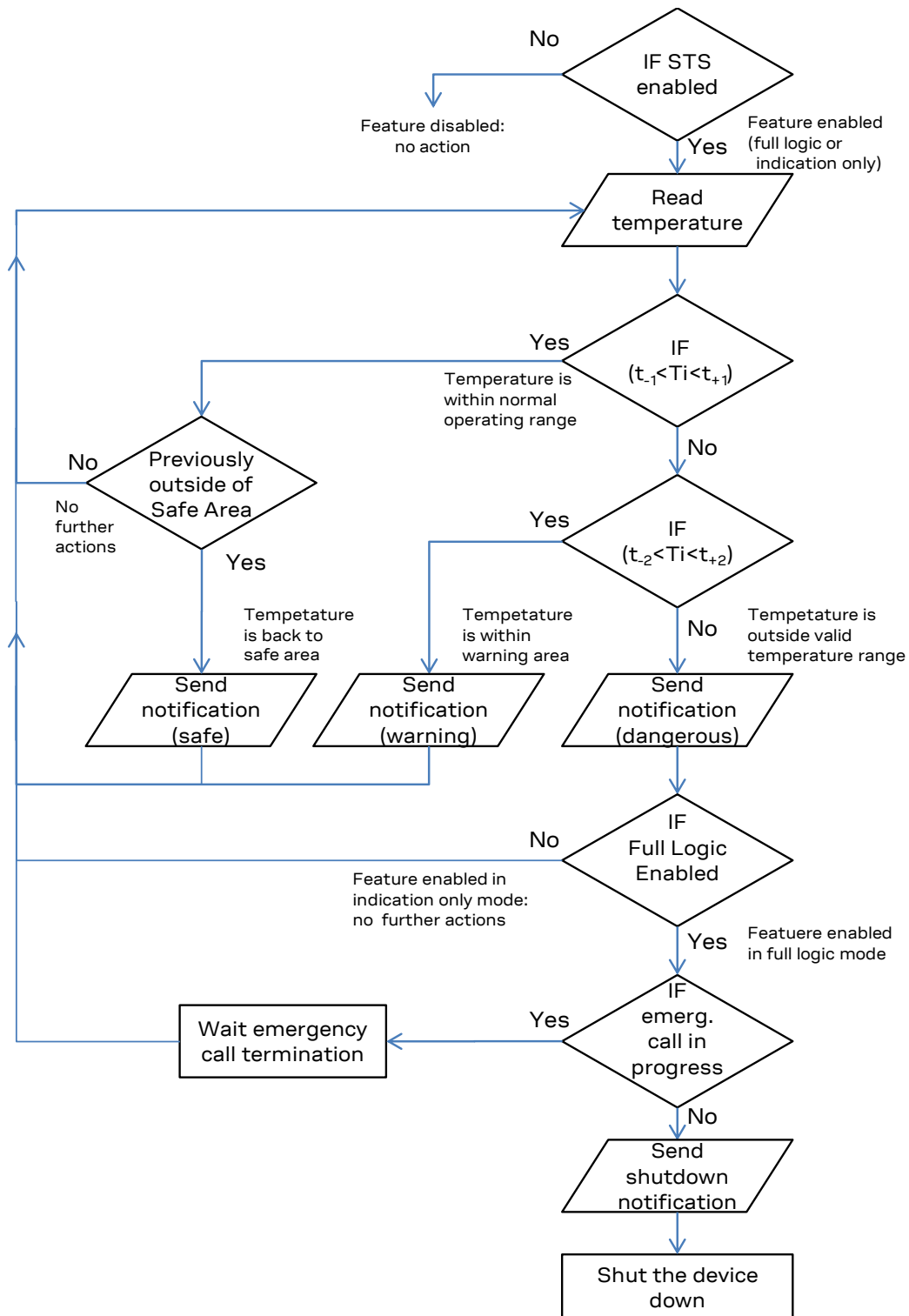
Figure 26: Smart Temperature Supervisor (STS) flow diagram
