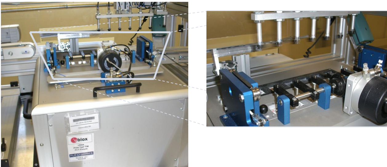
Figure 71: Automatic test equipment for module tests
