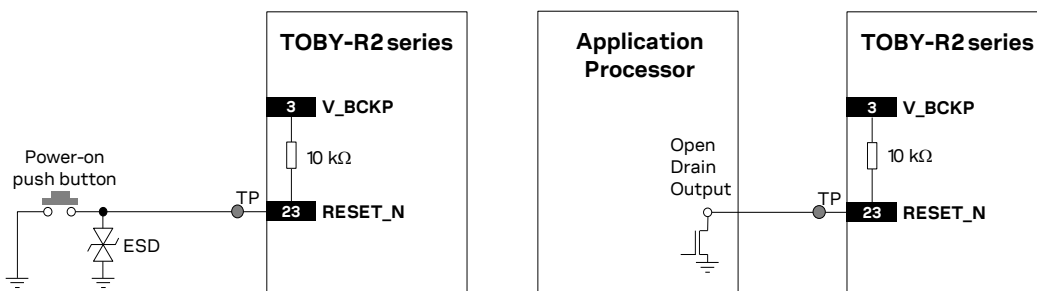
Figure 40: RESET_N application circuits using a push button and an open drain output of an application processor
