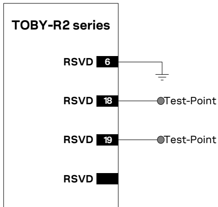
Figure 67: Application circuit for the reserved pins (RSVD)
