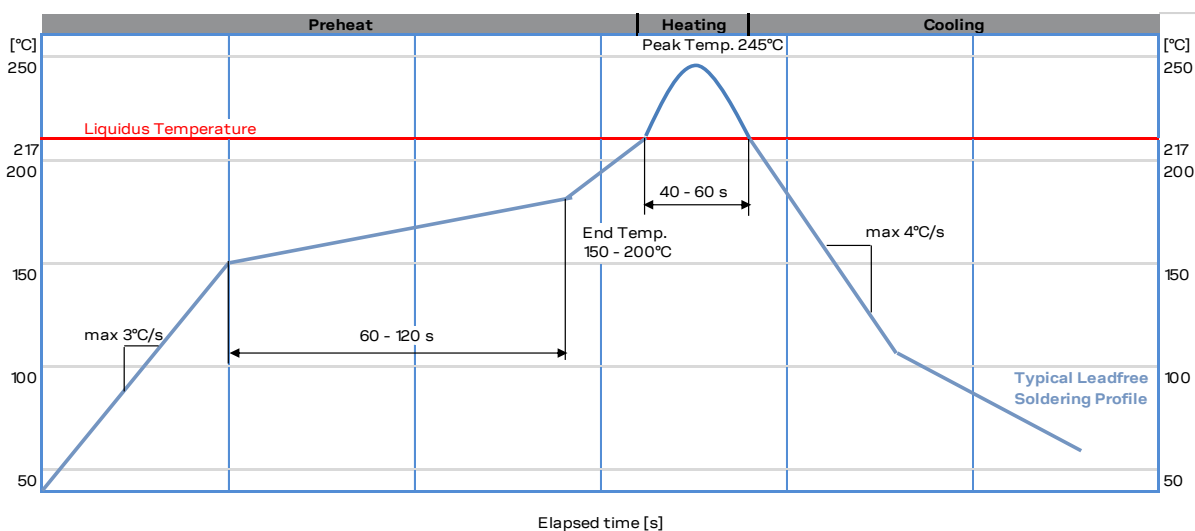
Figure 70: Recommended soldering profile
