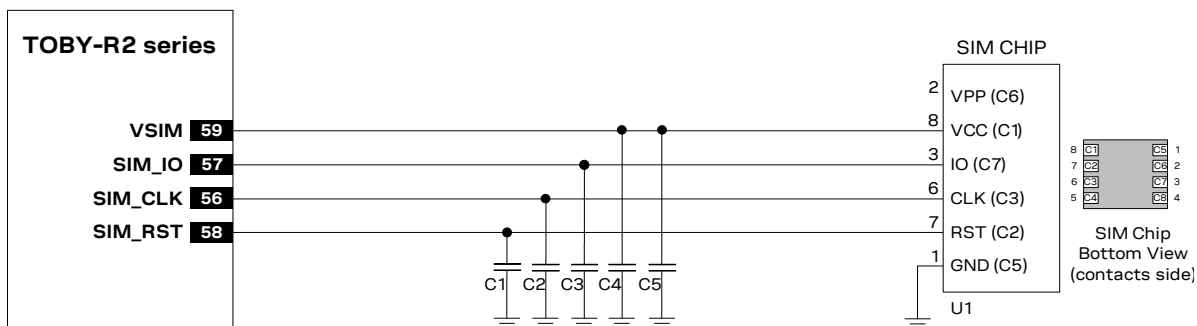
Figure 48: Application circuits for the connection to a single solderable SIM chip, with SIM detection not implemented
