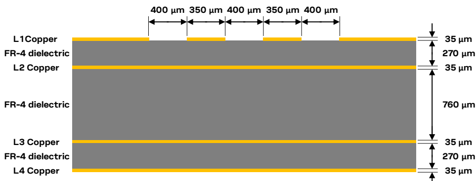
Figure 60: Example of USB line design, with Z_0 close to 90\ \Omega and Z_{CM} close to 30\ \Omega , for the described 4-layer board layout
