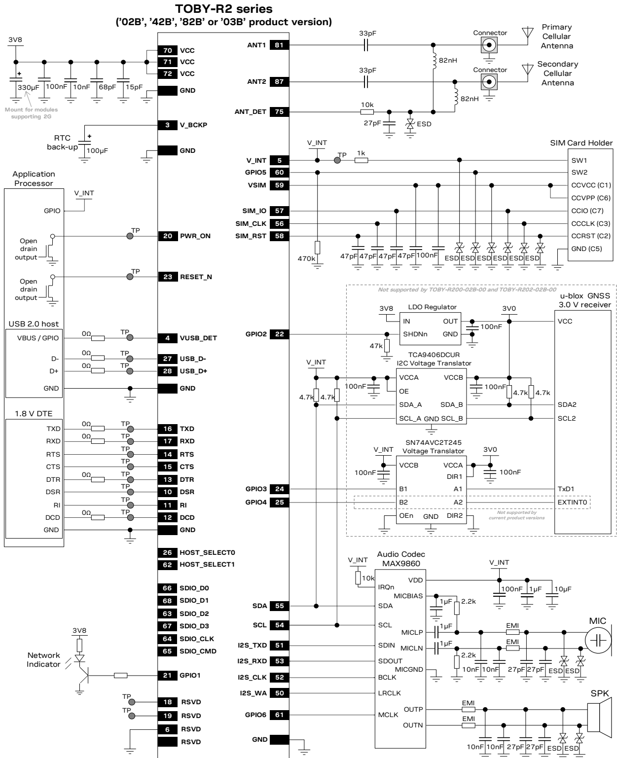
Figure 69: Example of schematic diagram to integrate a TOBY-R2 module "x2" product version using all available interfaces
