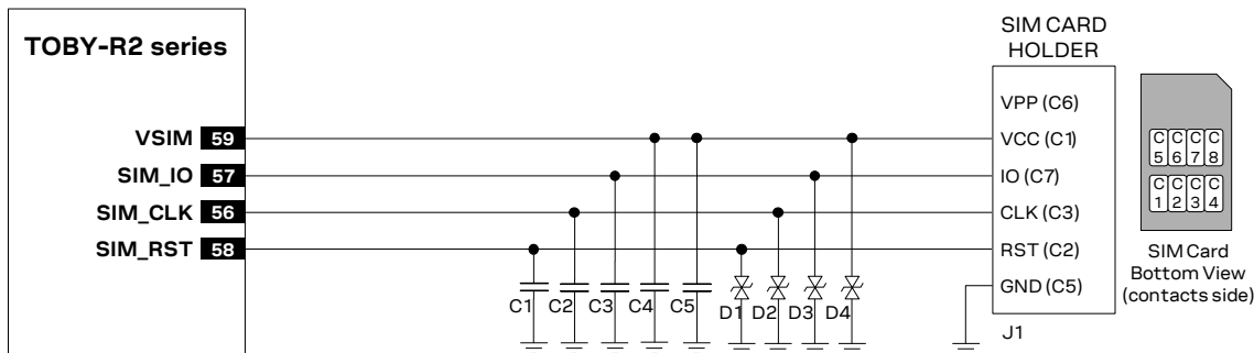
Figure 47: Application circuits for the connection to a single removable SIM card, with SIM detection not implemented
