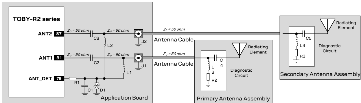
Figure 46: Suggested schematic for antenna detection circuit on application PCB and diagnostic circuit on antenna assembly
