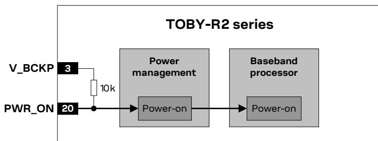
Figure 13: TOBY-R2 series PWR_ON input description
