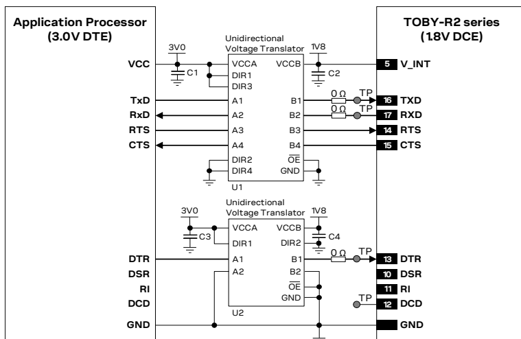
Figure 54: UART interface application circuit with partial V.24 link (6-wire) in DTE/DCE serial communication (3.0 V DTE)
