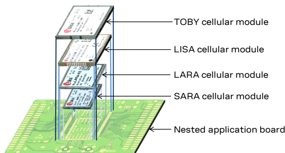
Figure 74: TOBY, LISA, SARA, LARA modules' layout compatibility: all modules are placed on the same nested footprint
