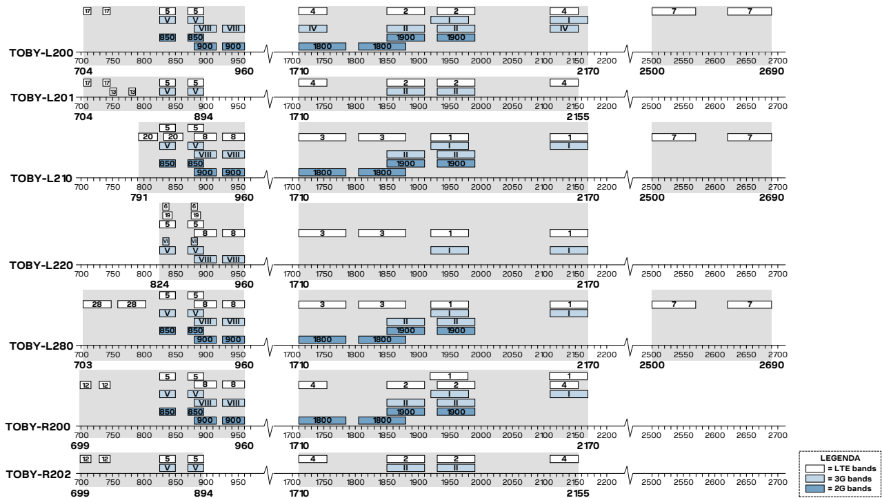
Figure 75: Summary of TOBY-L2 and TOBY-R2 series modules LTE, 3G and 2G operating frequency bands
