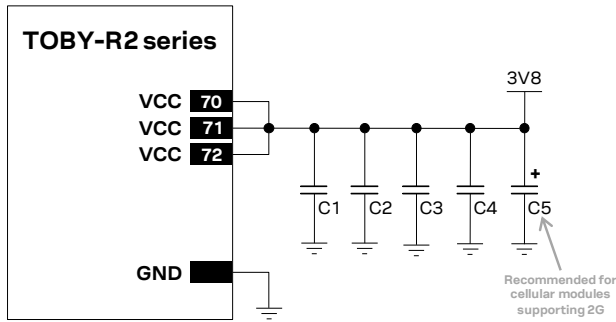
Figure 32: Suggested schematic for the VCC bypass capacitors to reduce ripple / noise on supply voltage profile
