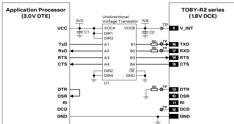
Figure 56: UART interface application circuit with partial V.24 link (5-wire) in DTE/DCE serial communication (3.0 V DTE)
