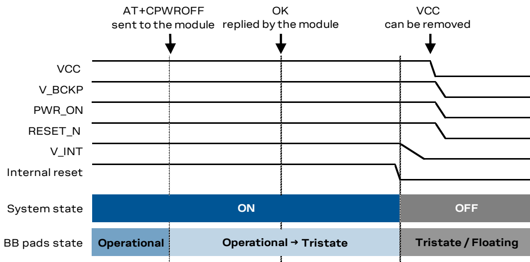
Figure 15: TOBY-R2 series switch-off sequence by means of AT+CPWROFF command
