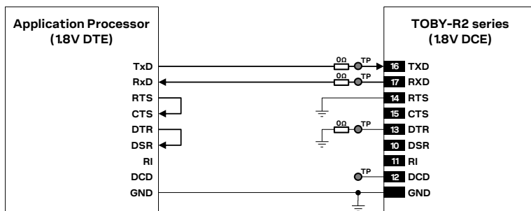
Figure 57: UART interface application circuit with partial V.24 link (3-wire) in the DTE/DCE serial communication (1.8V DTE)
