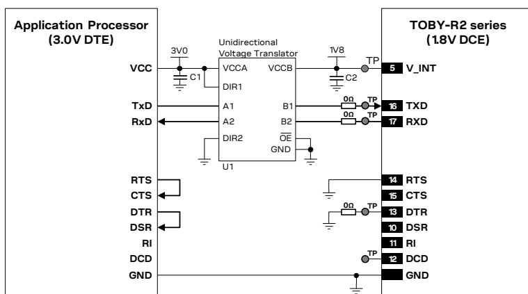
Figure 58: UART interface application circuit with partial V.24 link (3-wire) in DTE/DCE serial communication (3.0 V DTE)
