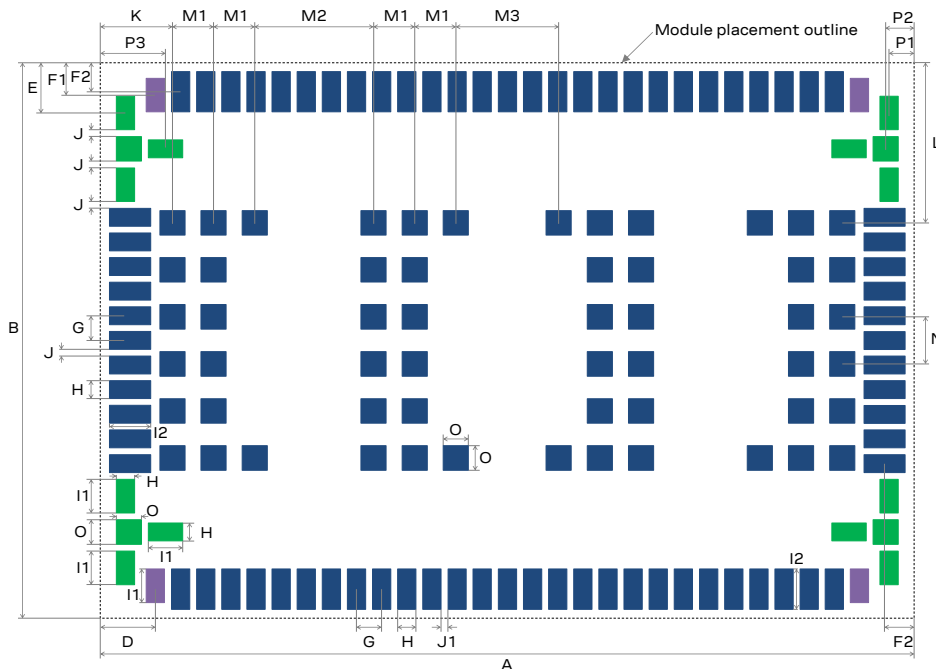
Figure 68: TOBY-R2 series module suggest footprint (application board top view)
