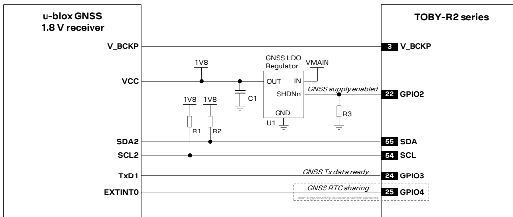
Figure 62: Application circuit for connecting TOBY-R2 series modules to u-blox 1.8 V GNSS receivers
