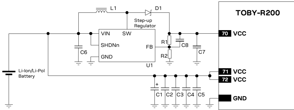
Figure 33: VCC circuit example with separate supply for TOBY-R200 modules
