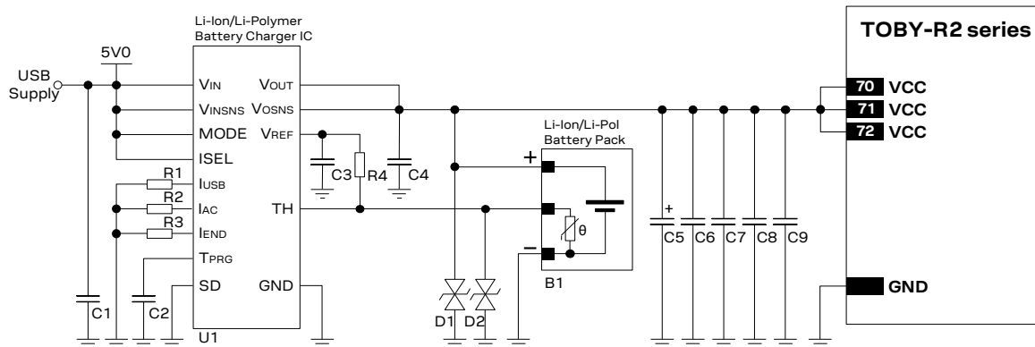
Figure 34: Li-Ion (or Li-Polymer) battery charging application circuit
