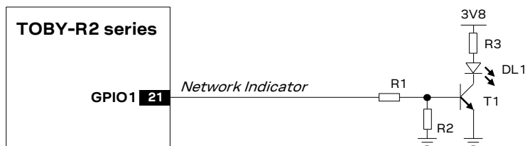
Figure 66: Application circuit for network indication provided over GPIO1
