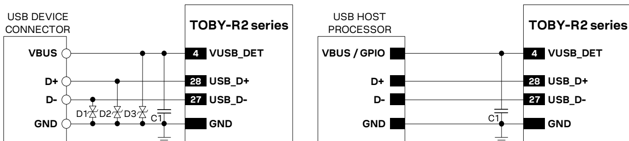
Figure 59: USB Interface application circuits
