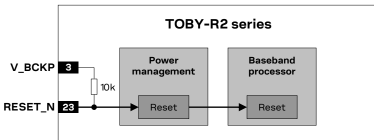
Figure 17: TOBY-R2 series RESET_N input equivalent circuit description
