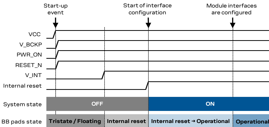
Figure 14: TOBY-R2 series switch-on sequence description
