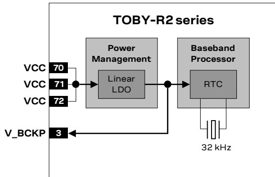
Figure 11: TOBY-R2 series RTC supply (V_BCKP) simplified block diagram
