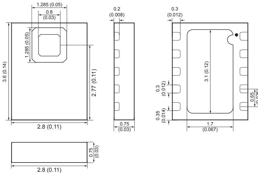
Figure 2: Dimensions
