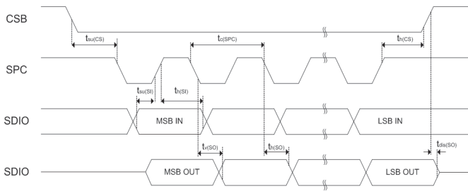
Figure 7: SPI slave timing diagram
