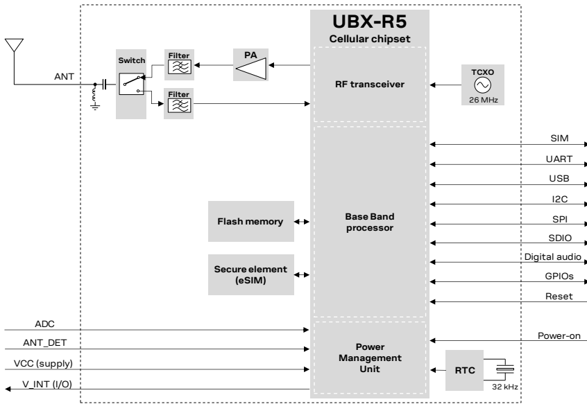
Figure 2: SARA-R510S block diagram
