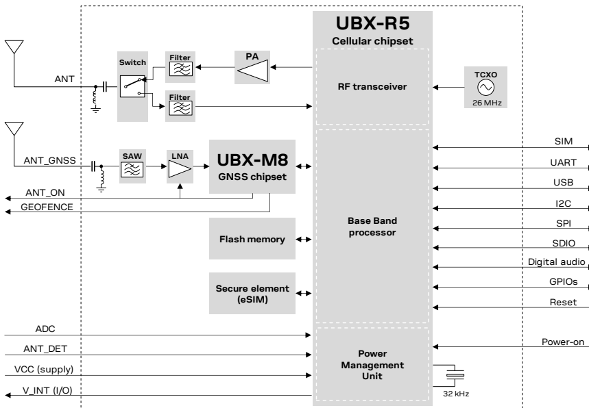
Figure 3: SARA-R510M8S block diagram
