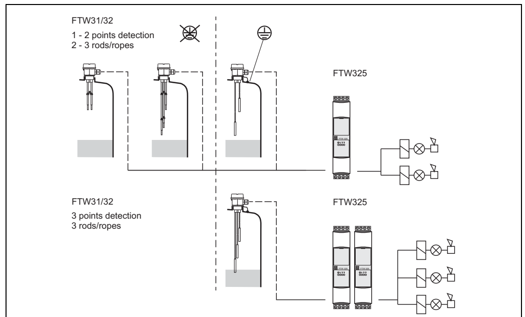
Switch points, depending on the tank material
