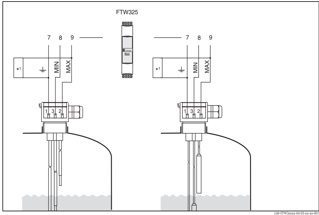
*1 Printed circuit board for cable monitoring (only required for probes with WHG certification.) The power supply and evaluation are provided by a switching unit, e.g. Nivotester FTW325
