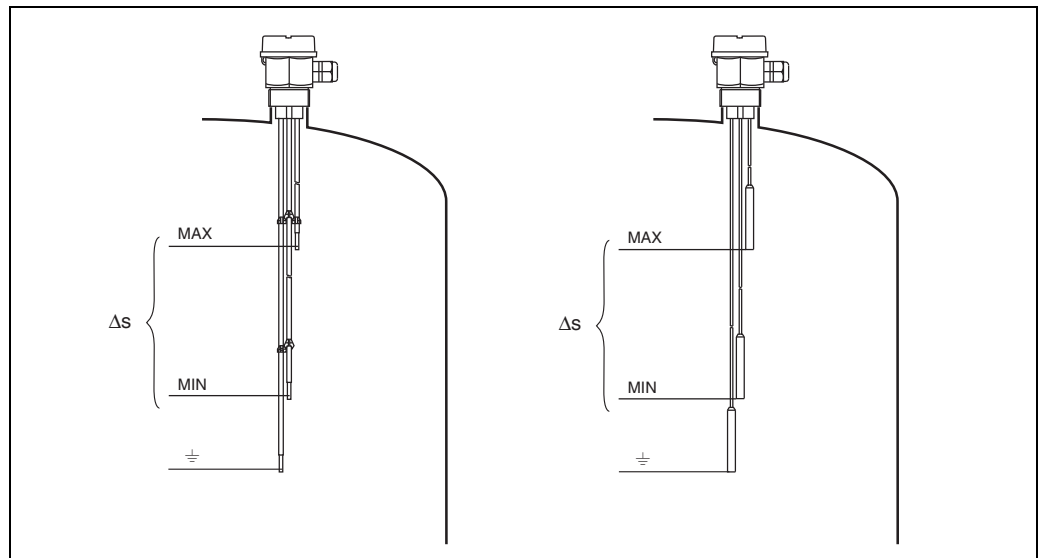
Two-point control ( \Delta s ) e.g. pump control
