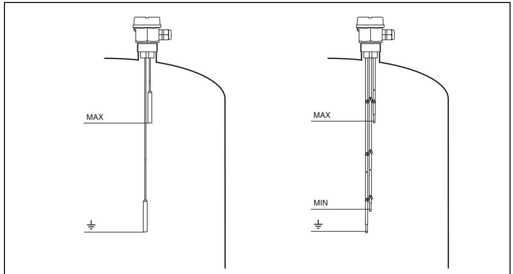
Point level detection (MAX), MAX and MIN detection for compact instrument version only possible with Δs.
