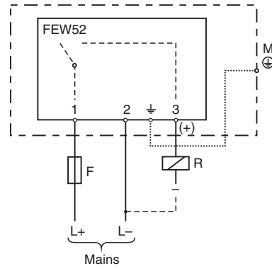
Connecting the FEW52 electronic insert F: Fine-wire fuse 500 mA, semi-time lag M: Ground connection to protective earth
