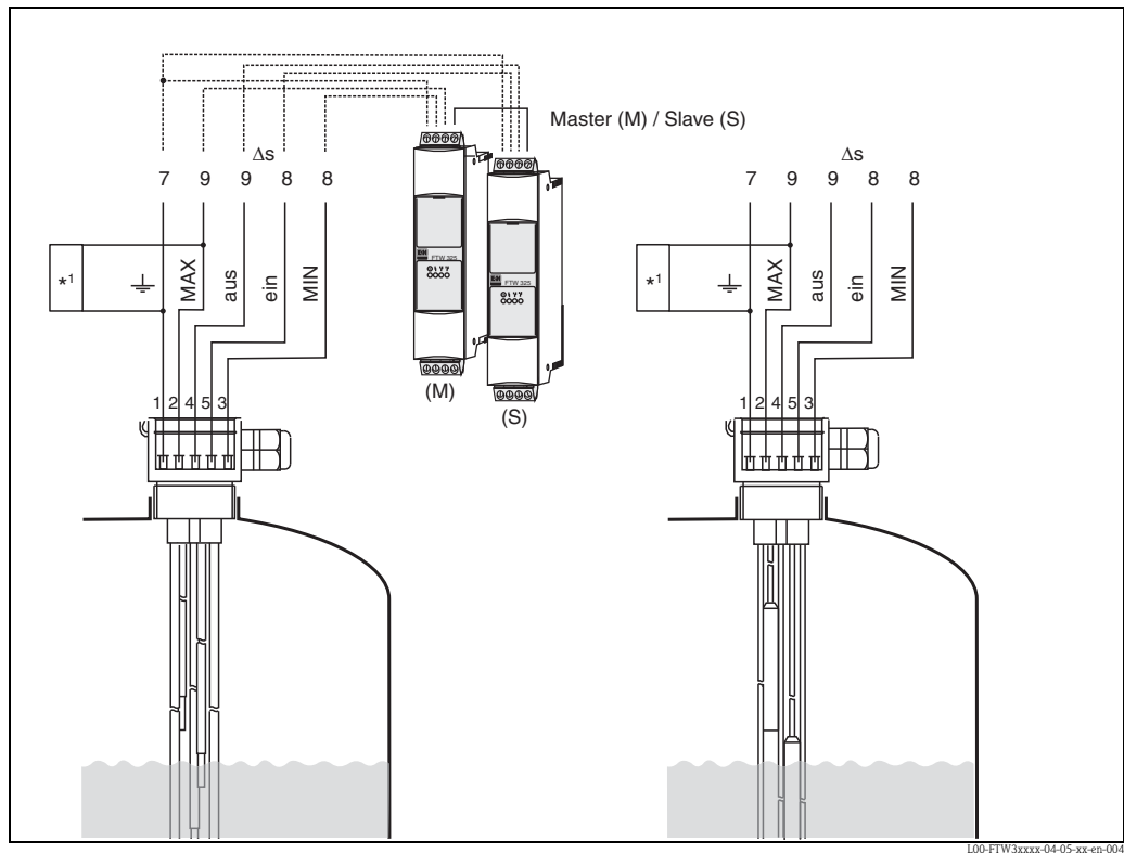
*1 Printed circuit board for cable monitoring (only required for probes with WHG certification.) The power supply and evaluation are provided by a switching unit, e.g. Nivotester FTW325
