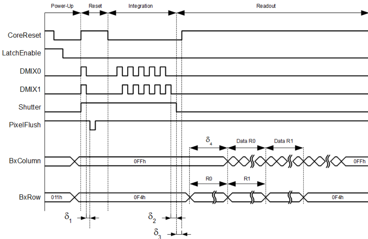
Figure 5: Global shutter timing \delta_1 \geq 0.1\mu s , \delta_2 \geq 0.1\mu s , \delta_3 \geq 1\mu s , \delta_4 \geq 1\mu s . Each cycle consists of a reset phase, an integration phase and a read-out phase.
