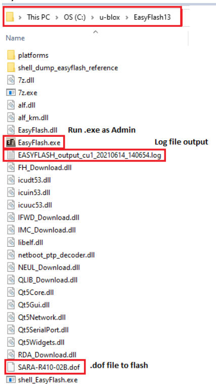
Figure 5: EasyFlash directory and file details
