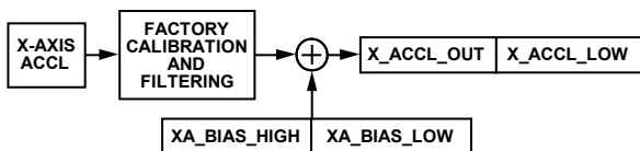
Figure 45. User Calibration Signal Path, Accelerometers
