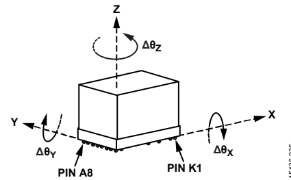
Figure 40. Delta Angle Axis and Polarity Assignments
