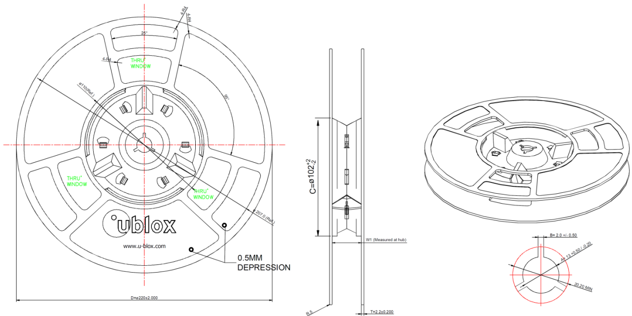
Figure 6: SARA-R4 series modules reel
